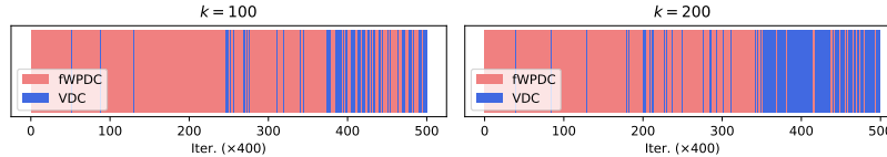
Fig. 7: Auto-selection result of the selector in the meta-joint optimization.
